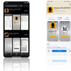
Mobile Apps
