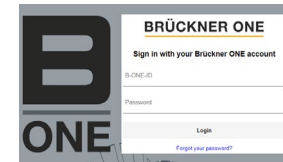
Single-sign-on
